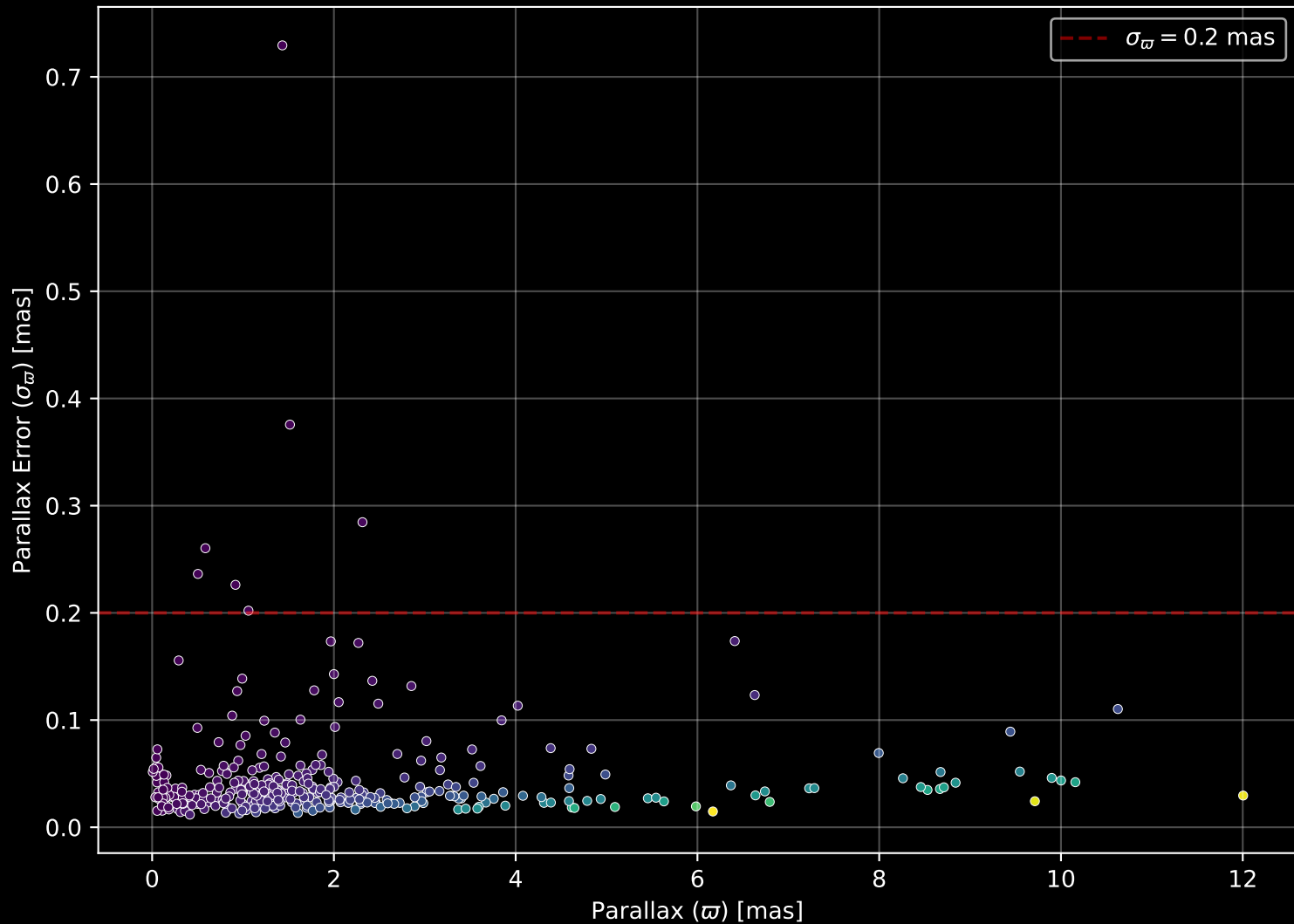
APOGEE DR17 Field: [ORPHAN-4] Parallax Quality (n= 345)
