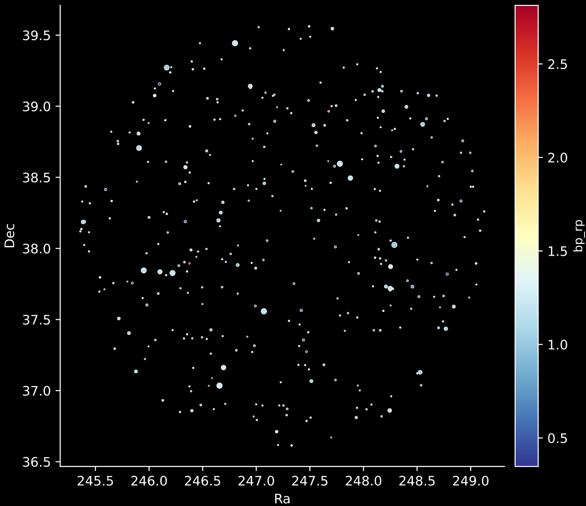
APOGEE DR17 Field: [ORPHAN-4] Stars: 345
