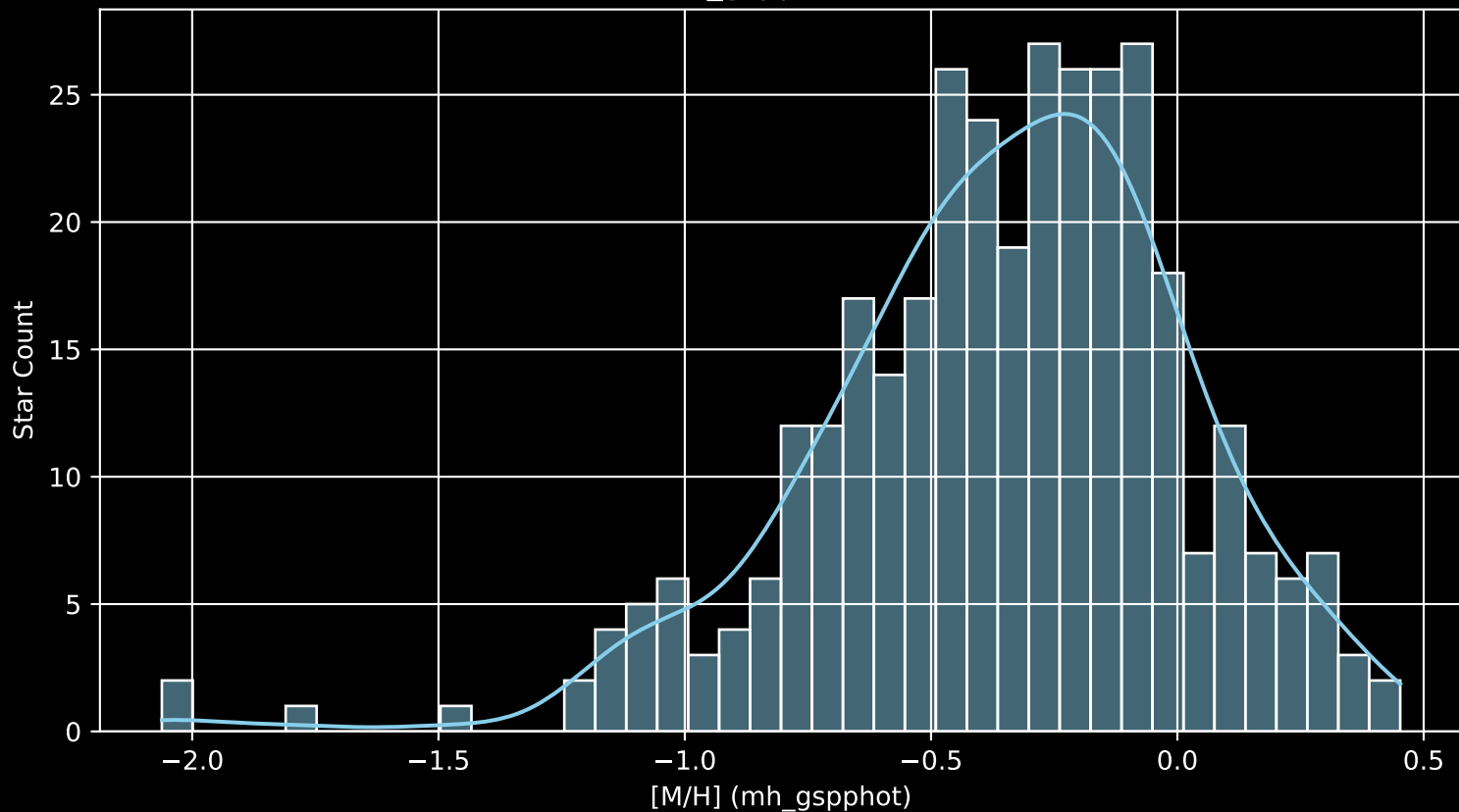
APOGEE DR17 Field: [ORPHAN-4 [M/H] (mh_gspphot) (n= 343)
