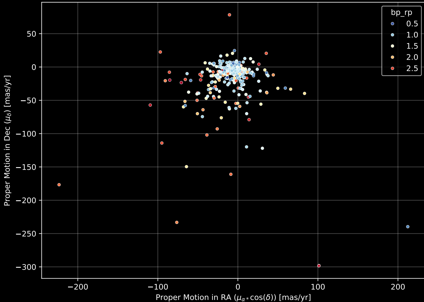
APOGEE DR17 Field: [ORPHAN-4] Proper Motion Diagram (n= 345)
