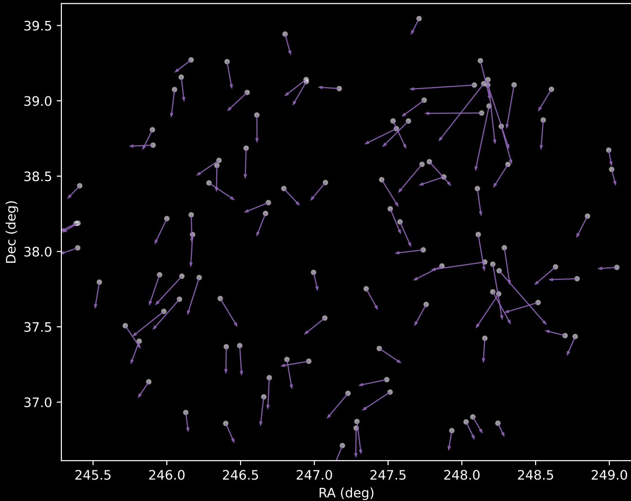
APOGEE DR17 Cluster 8 Proper Motion Vectors (n=103)
