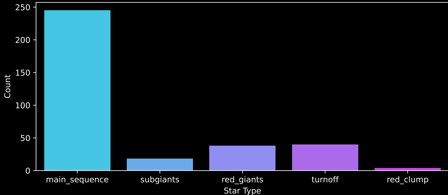
APOGEE DR17 Field: [ORPHAN-4] Count plot of Star Type
