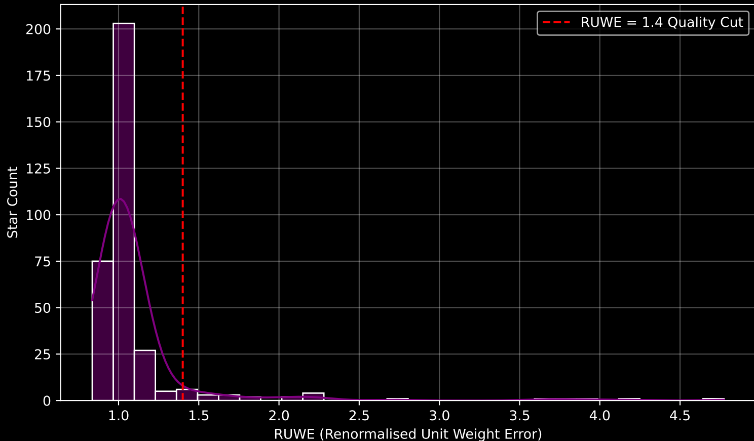
GAPOGEE DR17 Field [ORPHAN-4] RUWE Distribution (n= 336)
